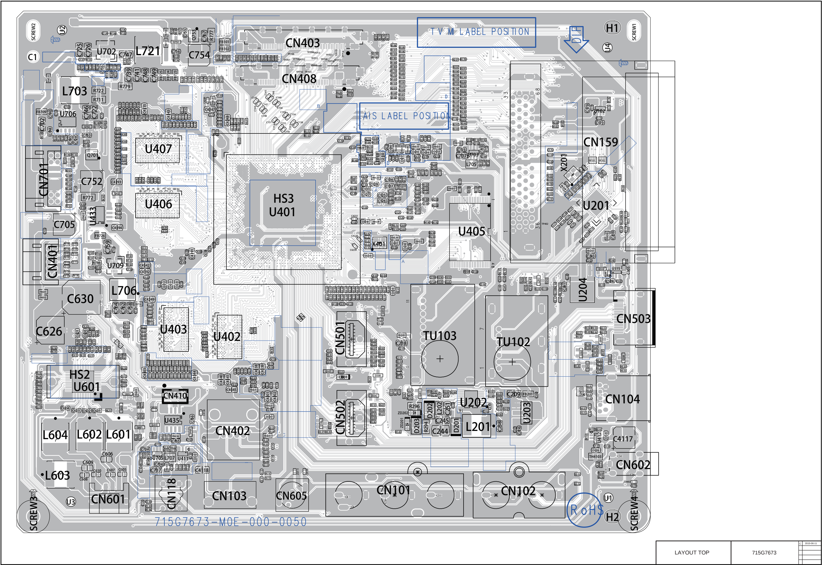
10-3-16 SSB layout top
