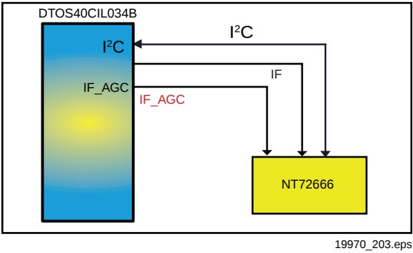
Figure 7-4 Front-End DVB-T/C DTV block diagram
