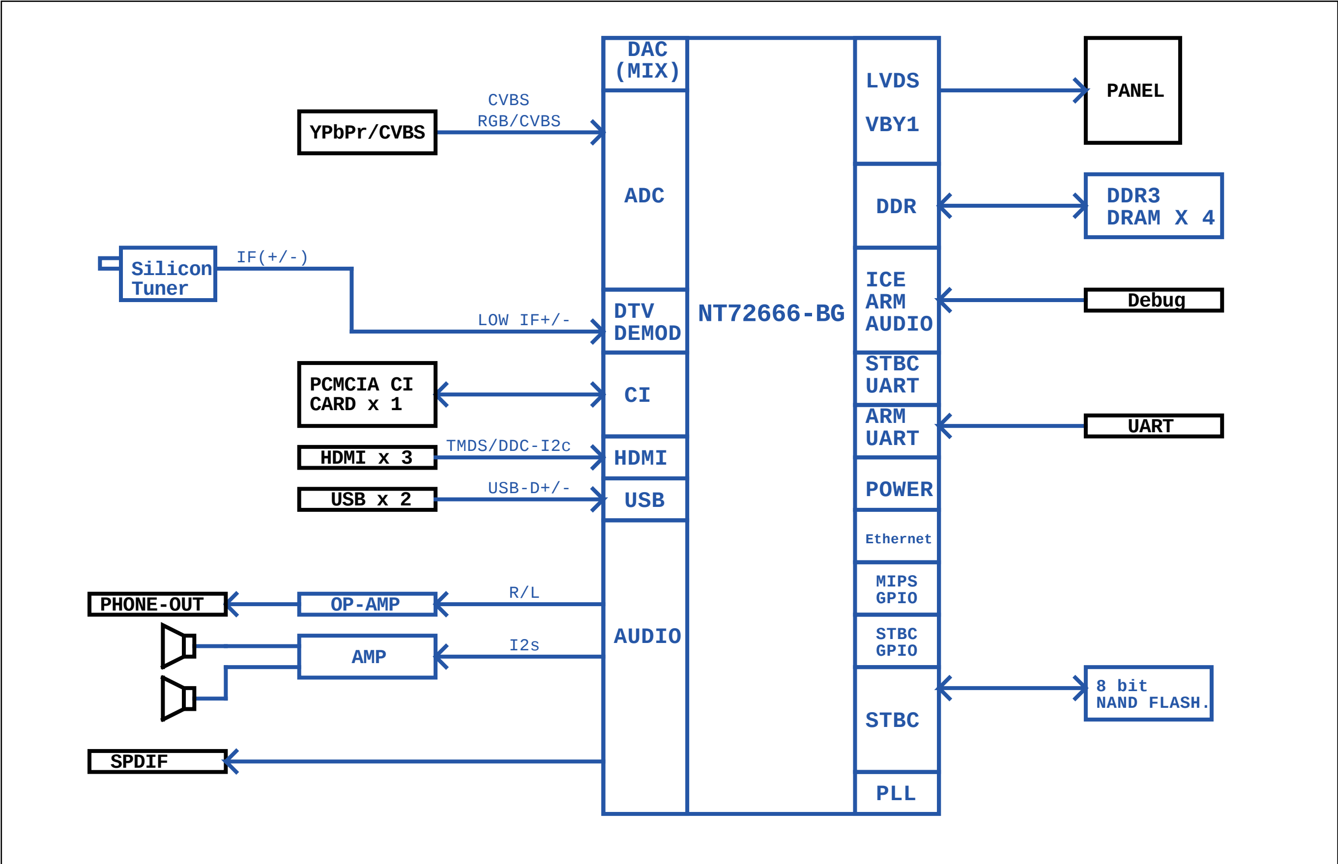
9.1 Block diagram 4900 series
