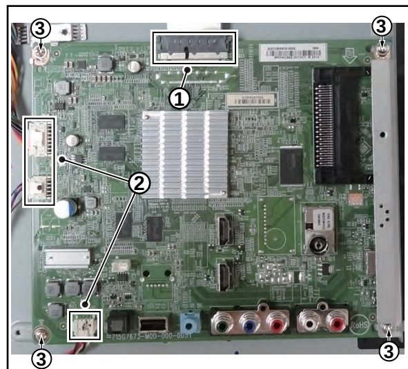
Figure 4-6 SSB removal
