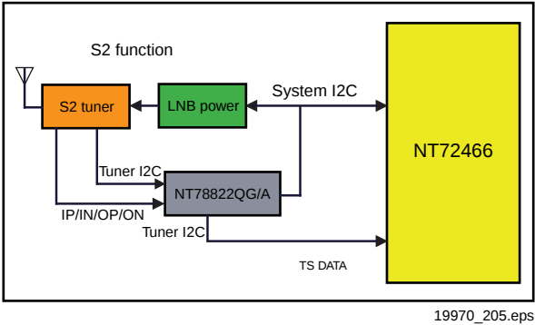
Figure 7-6 Front-End DVB-S2 DTV block diagram
