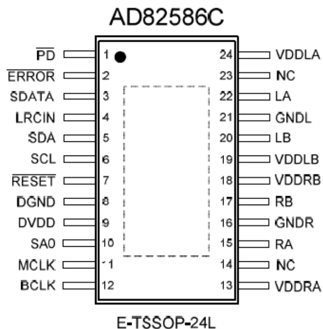
Figure 3.4: Pin description
