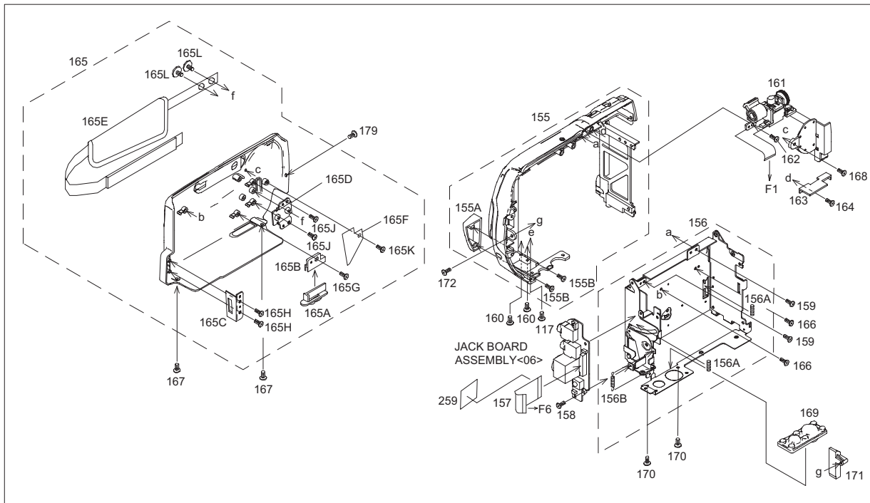
<LOWER ASSEMBLY>
