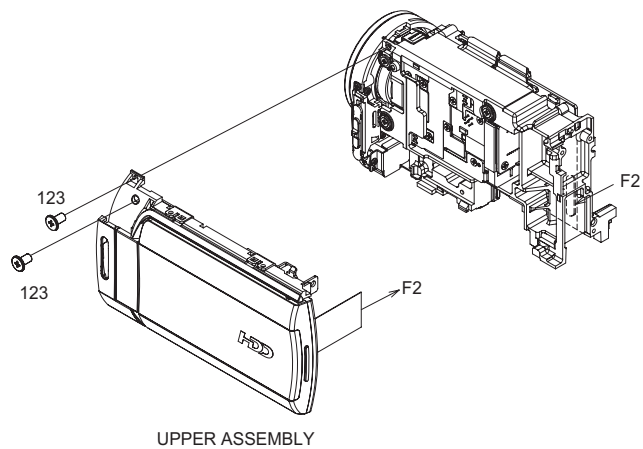
UPPER ASSEMBLY
