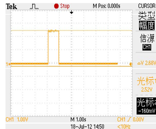
图9. XP11.12 AMP_MUTE
