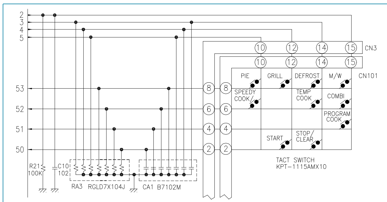
(key metrix and circuit diagram)
