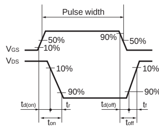
Fig.1-2 Switching Waveforms
