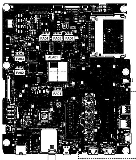
A PCB
