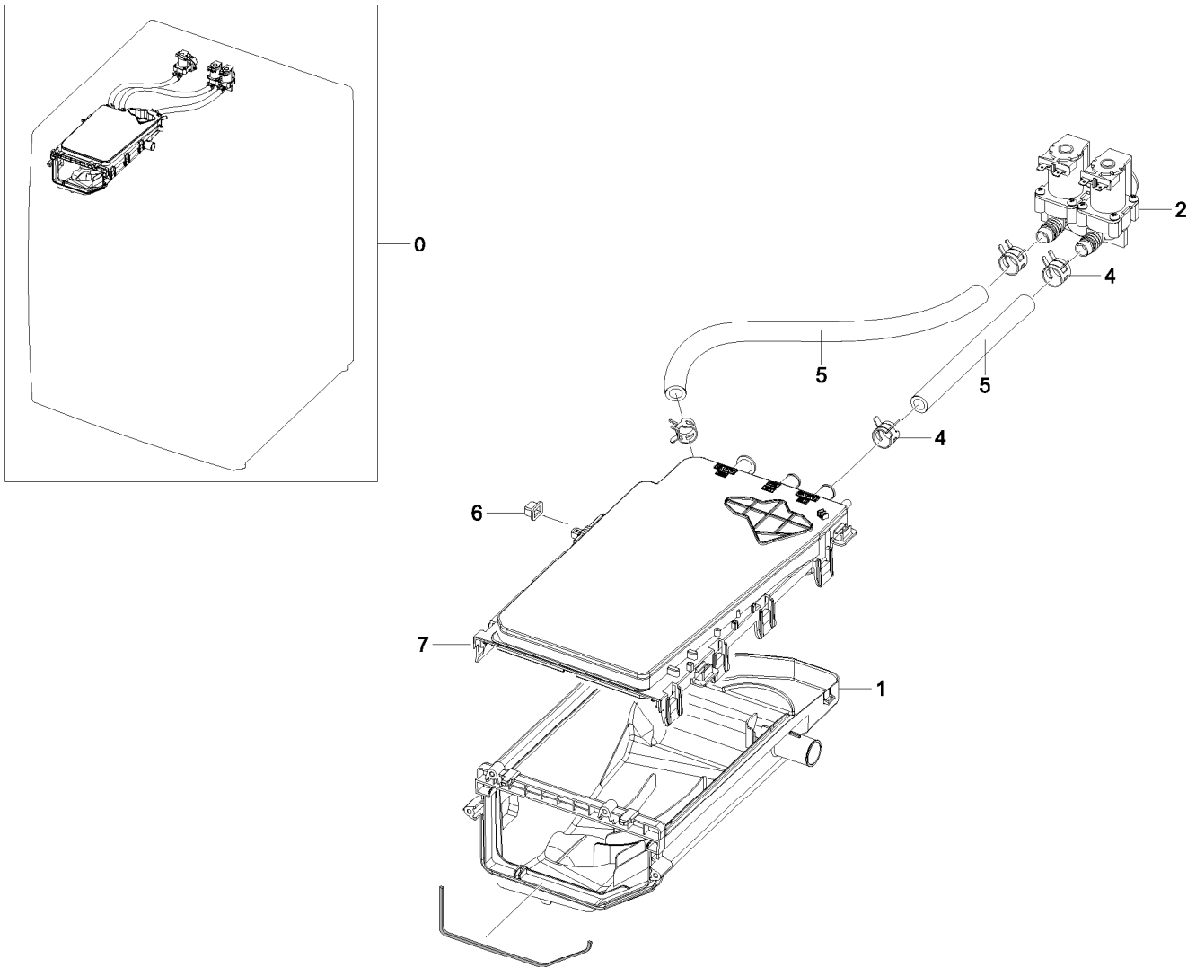
Exploded View
