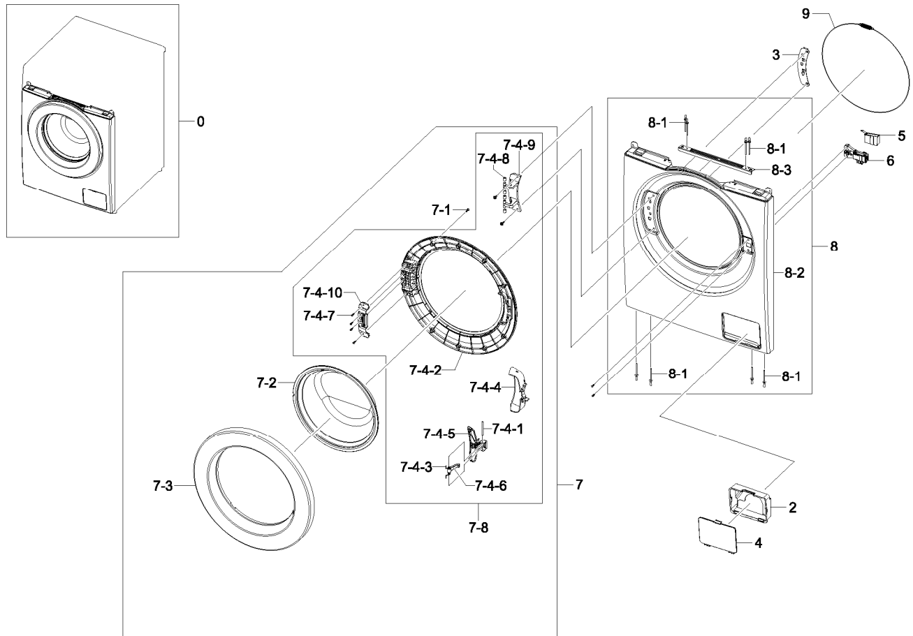
Exploded View
